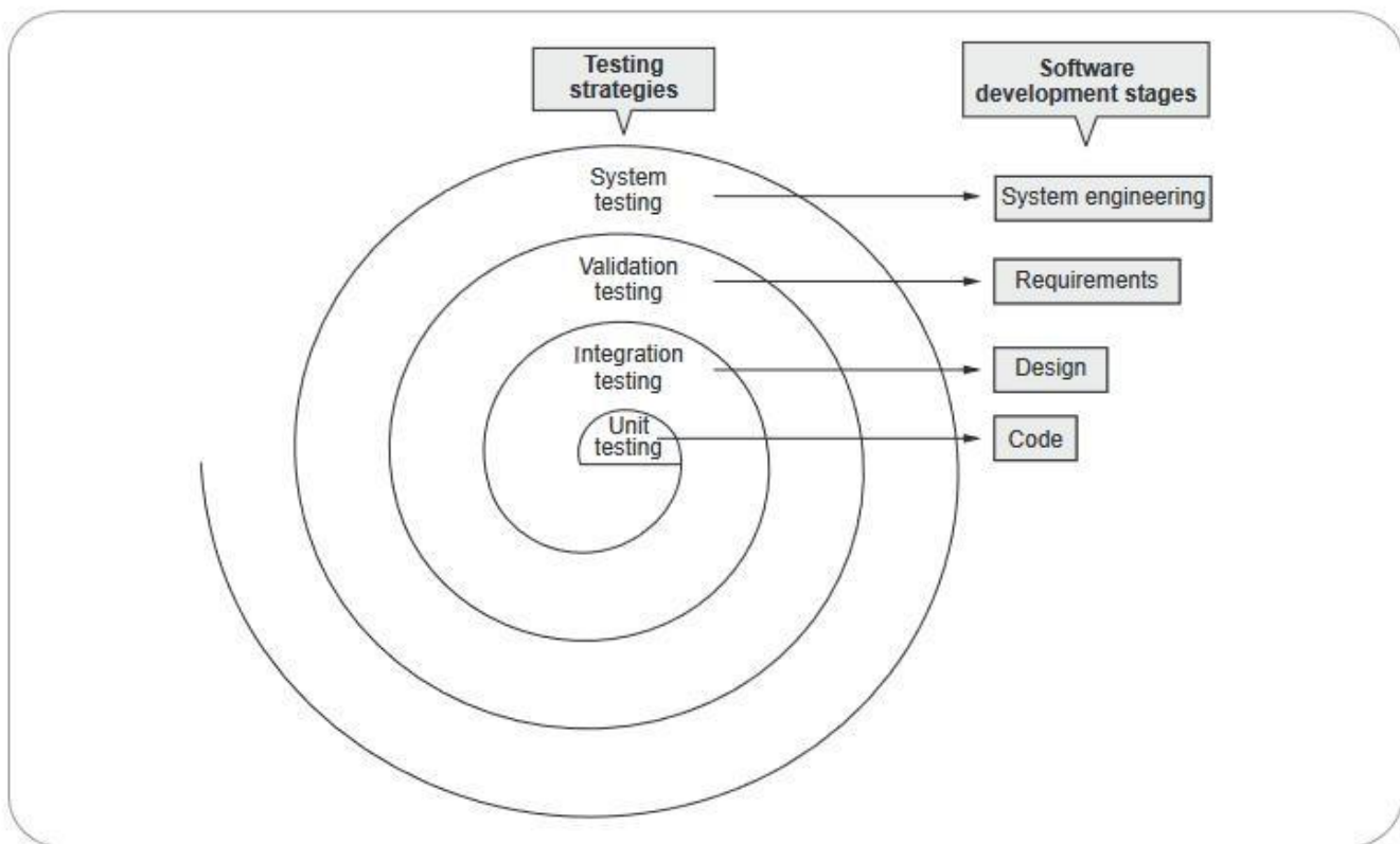
Fig. 3.5.1 Testing strategy
