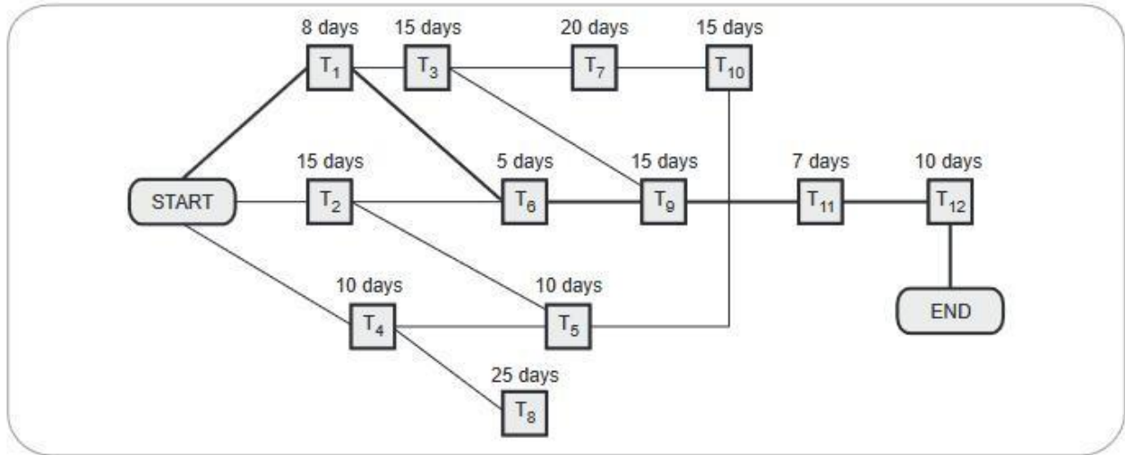
Fig. 5.1.4 Activity chart
