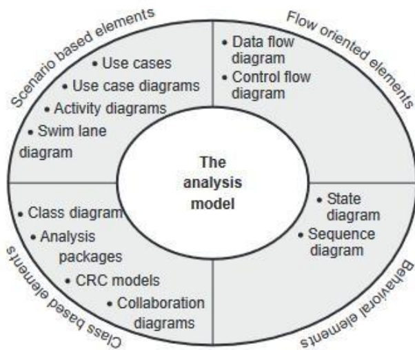
Fig. 3.2.1 Analysis model
