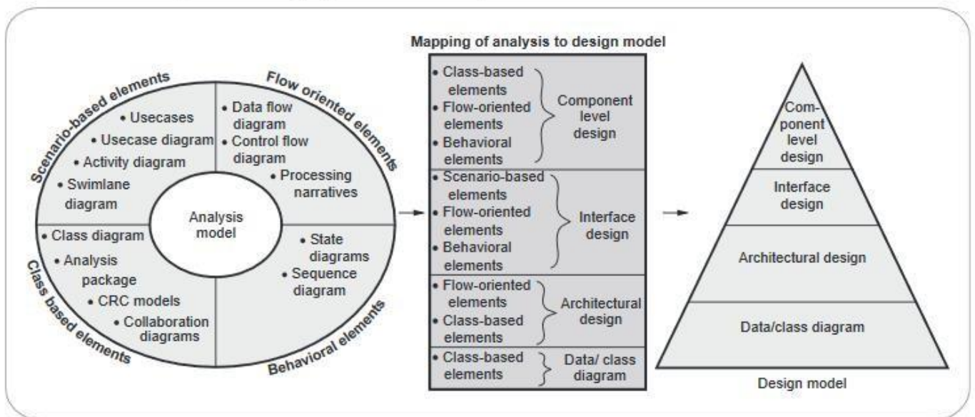
Fig. 3.1.1 Translating analysis model into the design model
