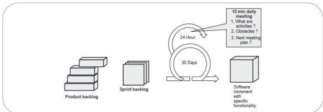
Fig. 1.8.3 SCRUM workflow activities
