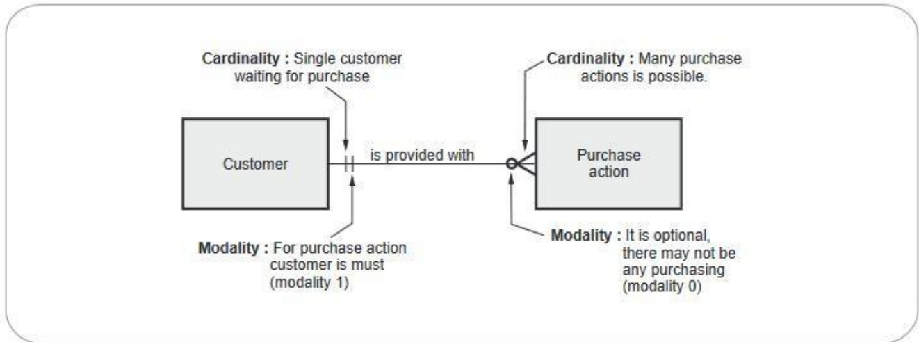
Fig. 3.1.3 Cardinality and modality
