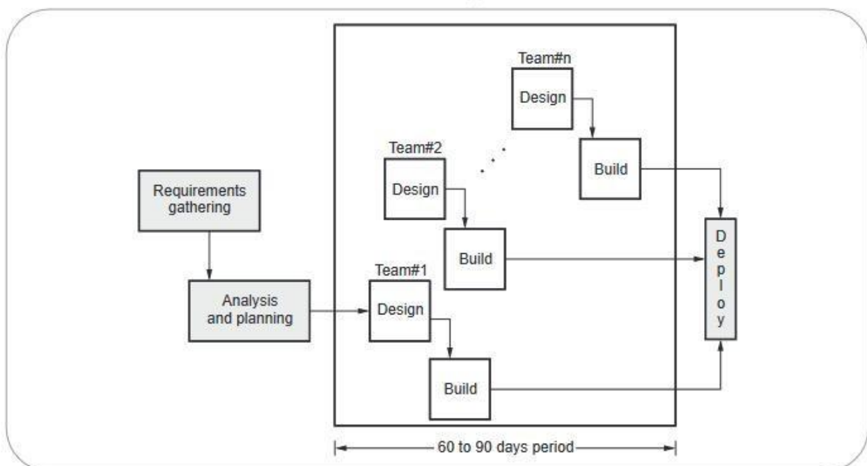
Fig. 1.7.3 RAD model
