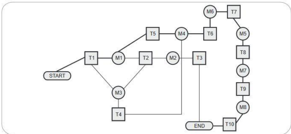
Fig. 5.1.3 Activity network
