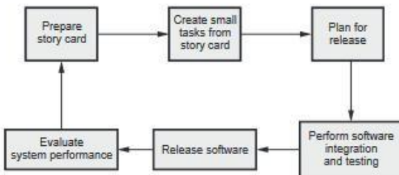
Fig. 1.8.1 Extreme programming release cycle
