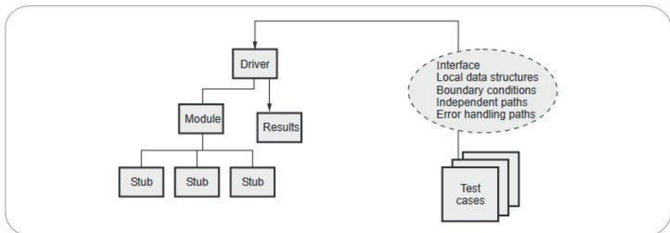
Fig. 3.5.3 Unit testing environment
