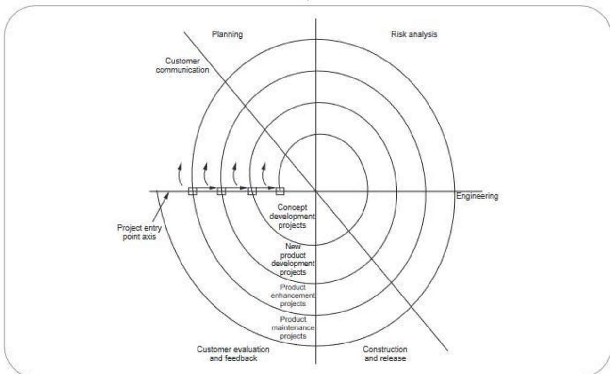
Fig. 1.7.4 Spiral model
