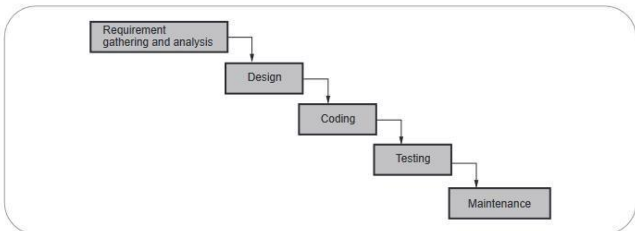
Fig. 1.7.2 Waterfall model
