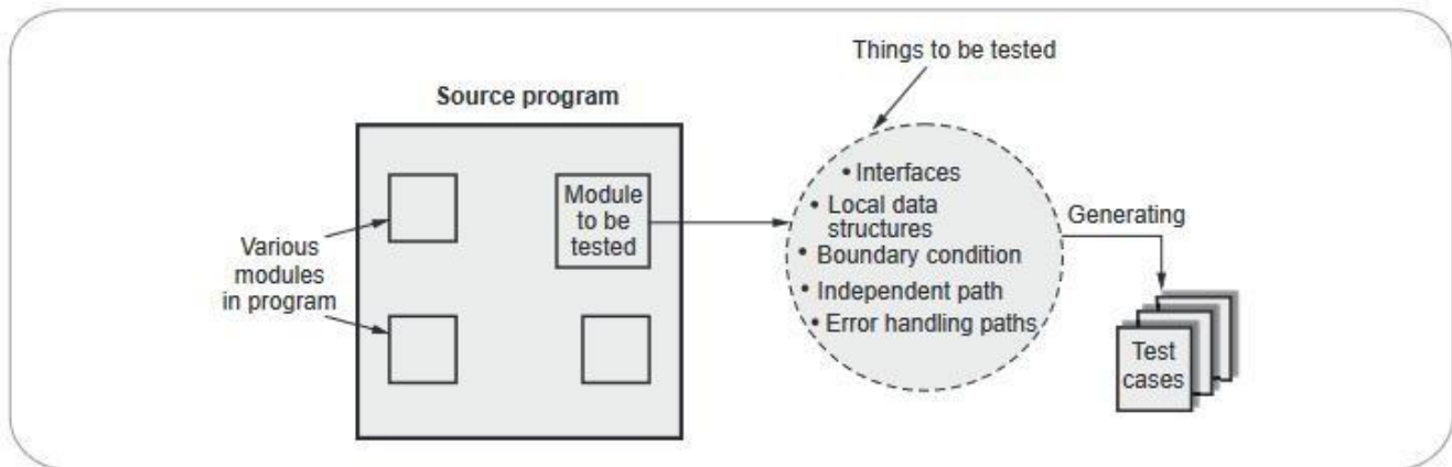
Fig. 3.5.2 Unit testing
